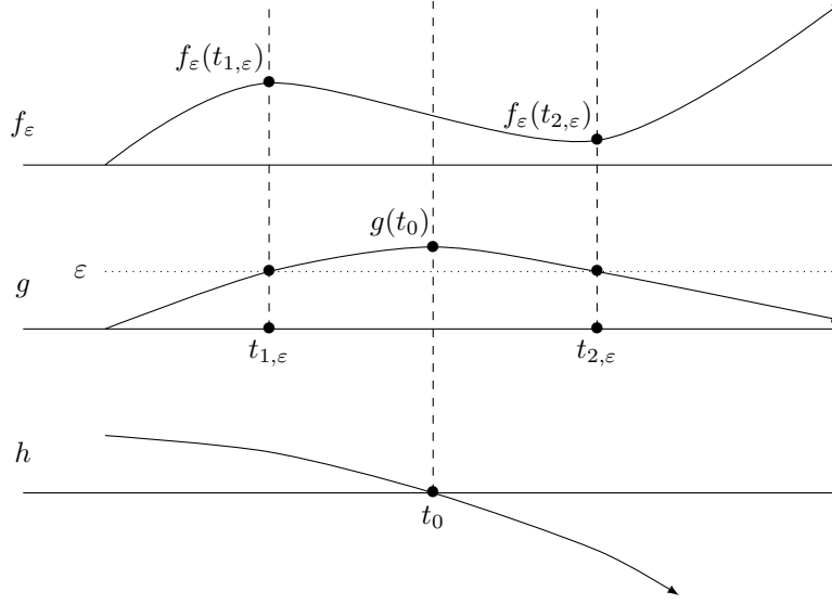
FIGURE 1. Functions in the proof of Lemma 3.1.
